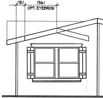
OPTION ENDWALL
