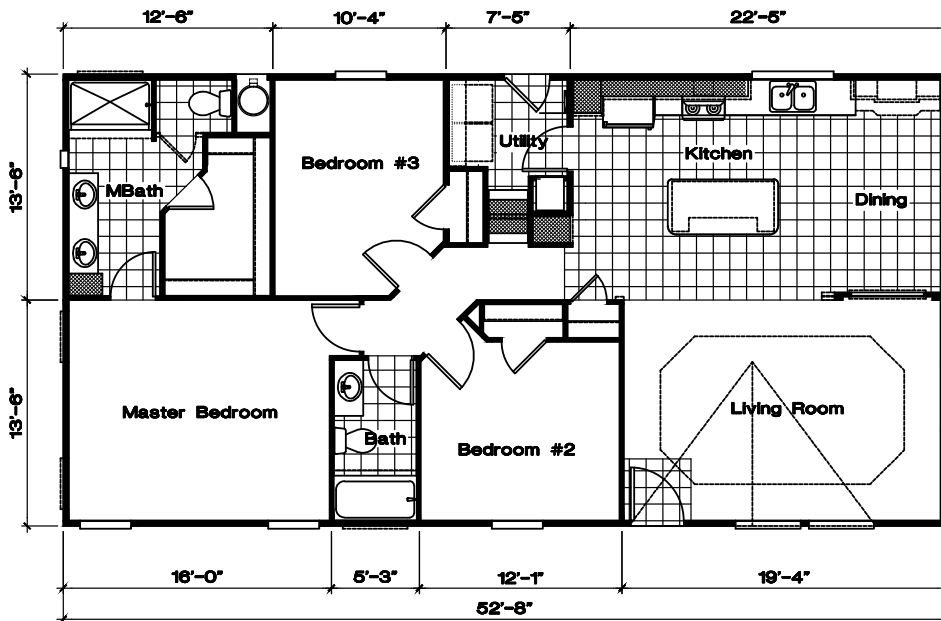
GLE528F STANDARD FLOOR PLAN
